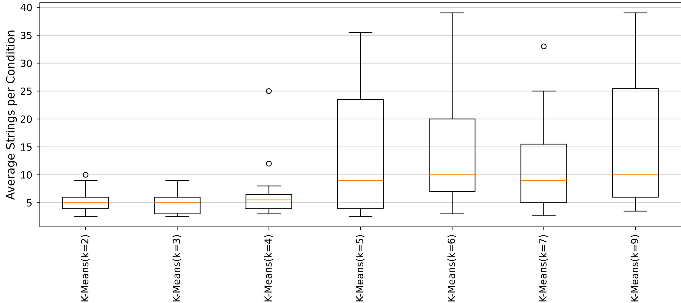
YARA Rules Average Strings per Condition Distribution (Cluster11_Size9 dataset)
